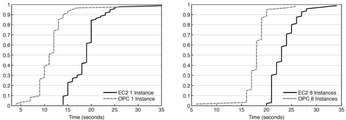
Figure 4. Empirical CDFs comparing number of seconds taken to start one and eight VM instances within EC2 and Eucalyptus.
